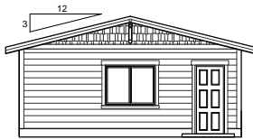
LEFT VIEW
