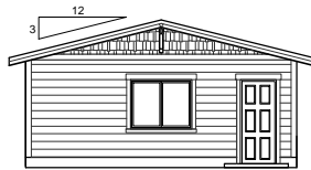
LEFT VIEW
